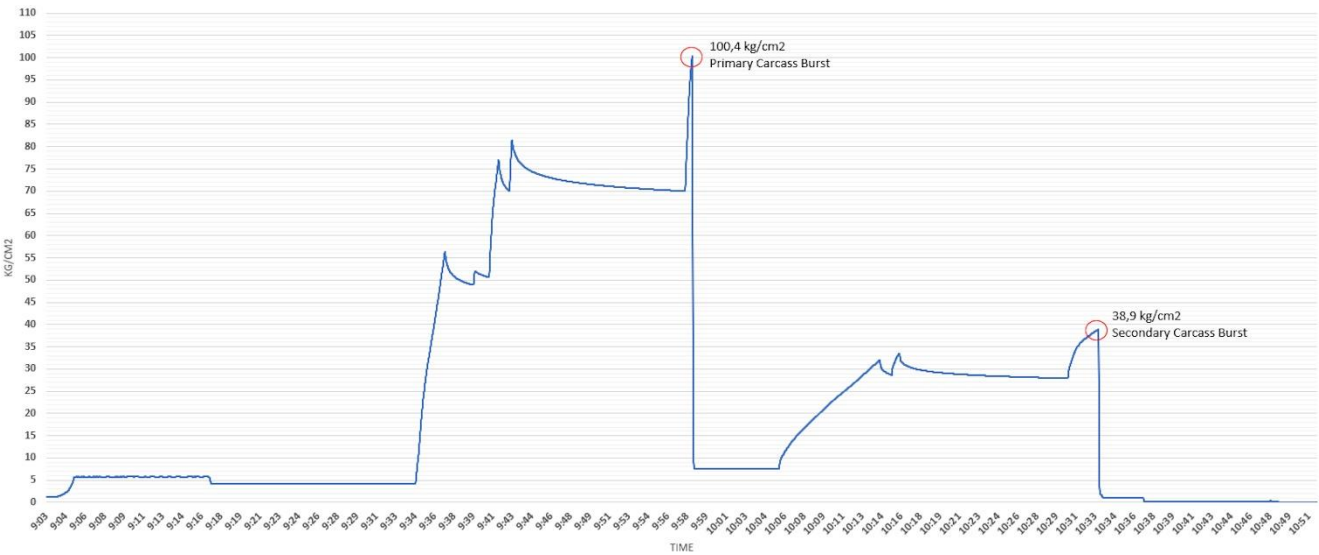
Mainline Subsea Hose Burst Test Graph - 19th June 2024
