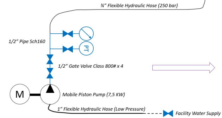
Burst Test Experimental Setup
